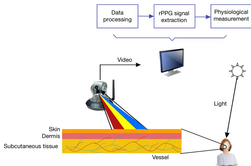
Figure 1. Schematic diagram of the rPPG principle. The figure illustrates the acquisition and processing of facial video for extracting physiological signals from subtle skin color variations associated with blood perfusion. Adapted from Chen et al. [7]. rPPG, remote photoplethysmography.
