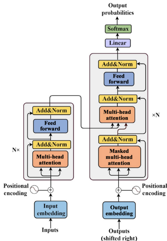
Figure 2. The transformer-model architecture. Figure displays the core structure of standard Transformer, focusing on multi-head self-attention mechanism which realizes global feature modeling. Reproduced from Vaswani et al. [5].
